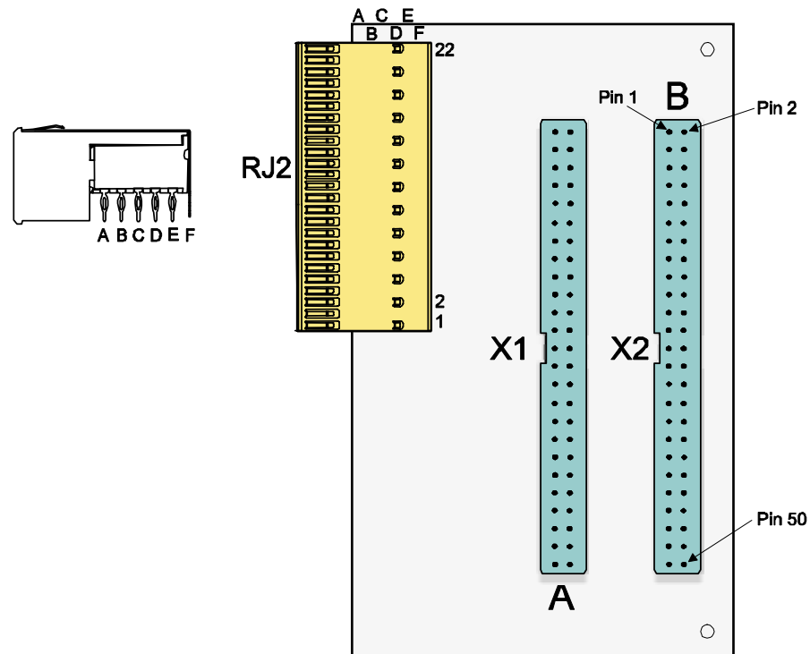
Figure 6-1 : Pin Assignment
