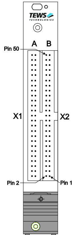
Figure 6-1 : I/O Pin Order
