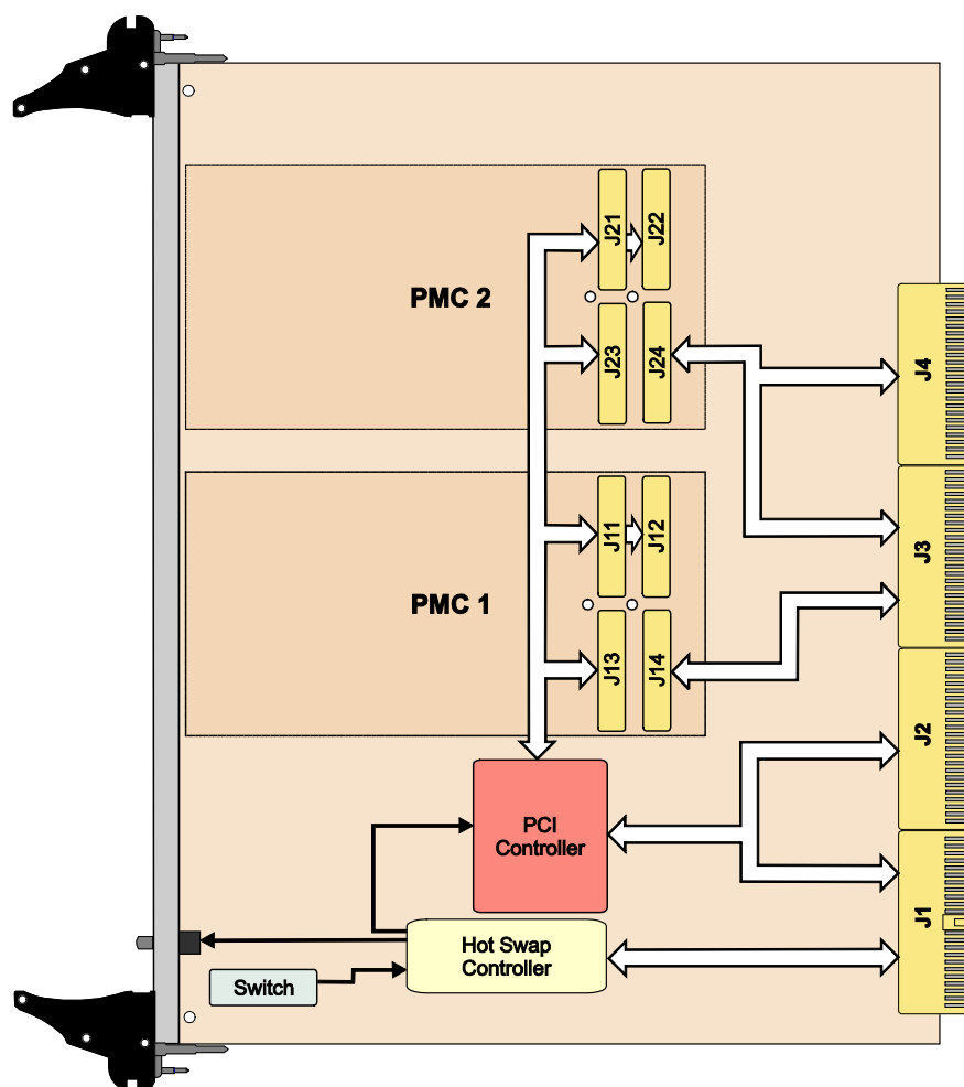
Figure 1-1 : Block Diagram
