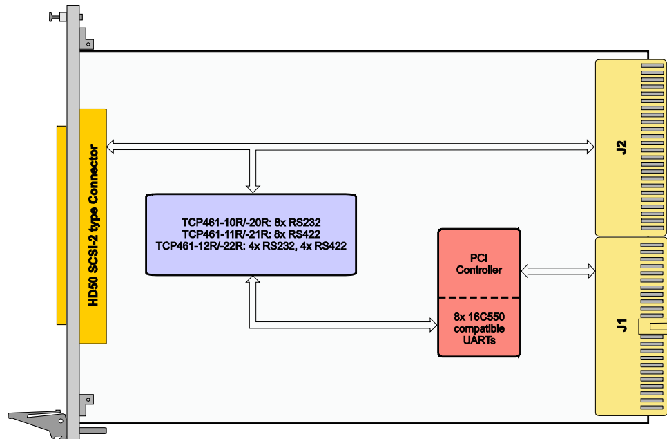
Figure 1-1 : Block Diagram
