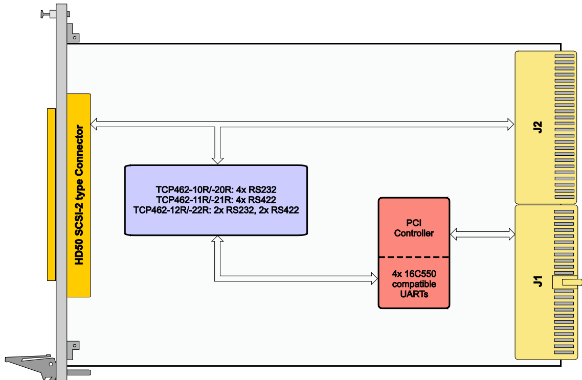
Figure 1-1 : Block Diagram
