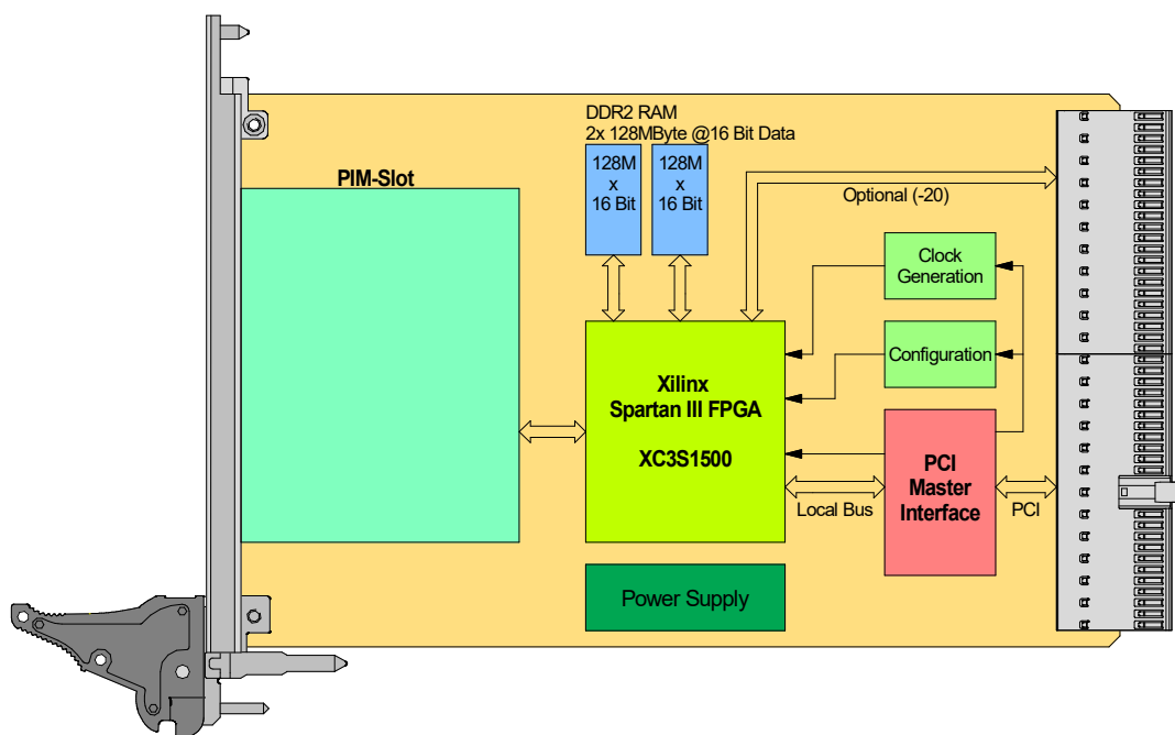
Figure 1-1 : Block Diagram
