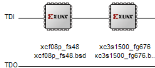
Figure 6-1 : This is how the JTAG-Chain should look like in iMPACT
