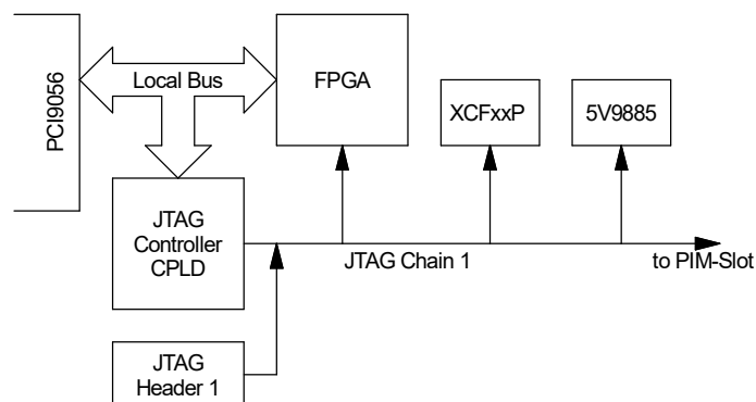
Figure 5-4 : In-System Programming
