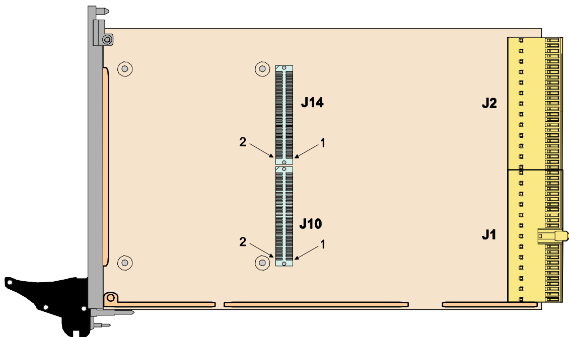
Figure 8-2 : Connector Positions
