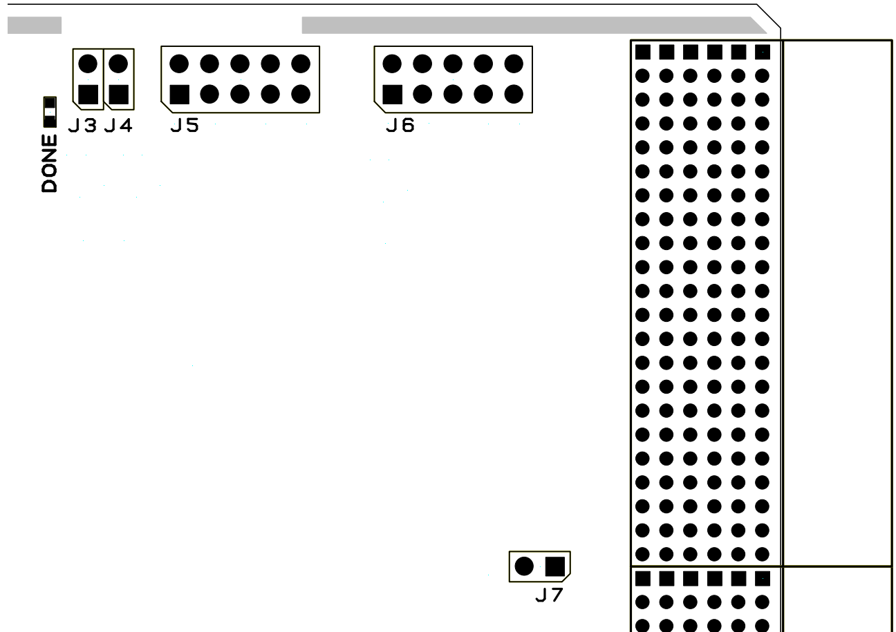
Figure 8-1 : Header & Jumper
