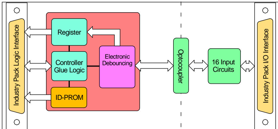
Figure 1-1 : Block Diagram
