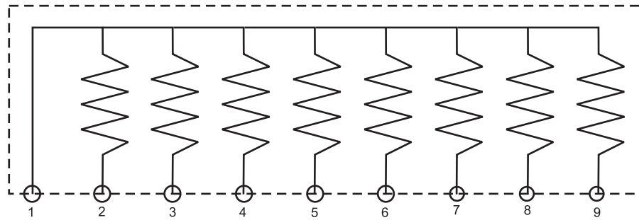
Figure 6-2 : Pining of Pull Up Resistors
