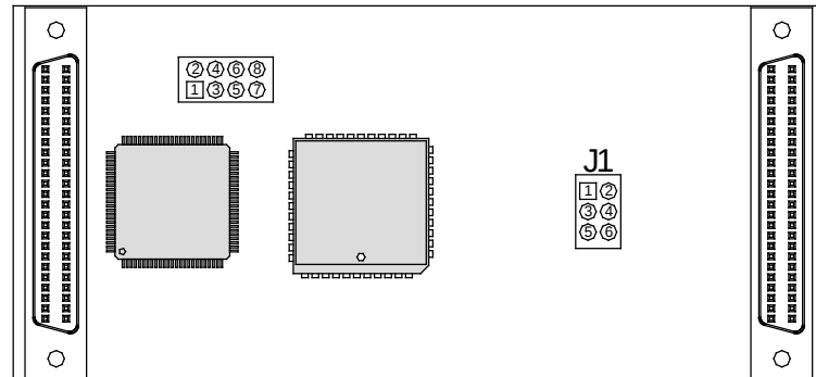
Figure 6-1 : Jumper Configuration
