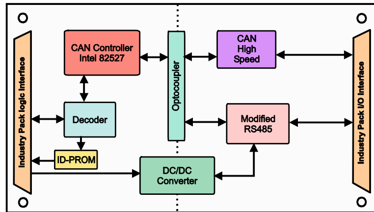
Figure 1-1 : Block Diagram
