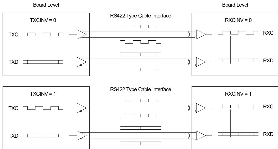
Figure 7-1 : Transmit & Receive Clock Polarity
