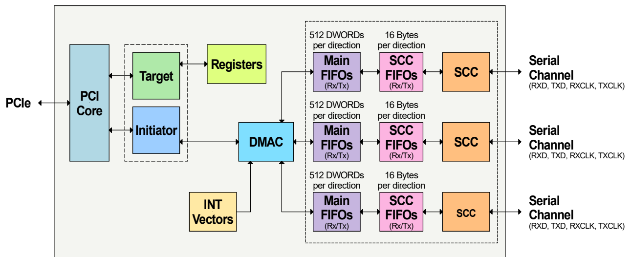
Figure 3-1 : FPGA On-Chip Block Diagram
