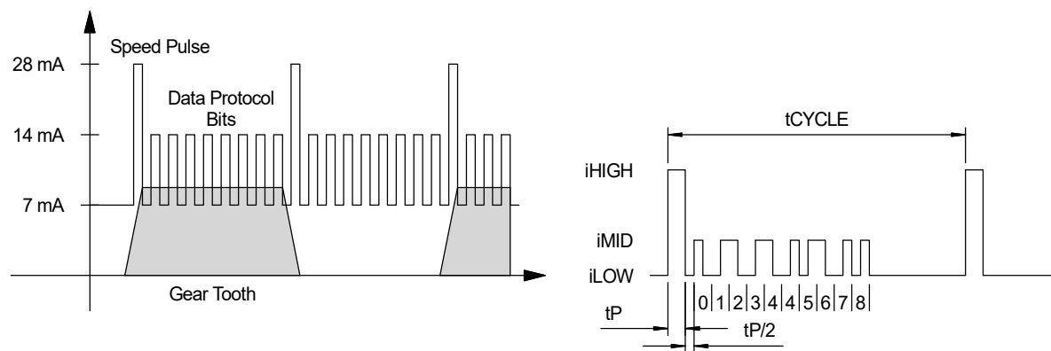
Figure 7-3 : AK-Protocol / VDA Diagram
