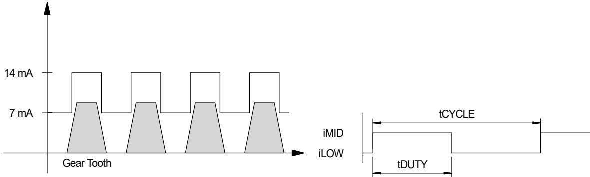
Figure 7-1 : Speed Protocol / Duty Cycle Diagram
