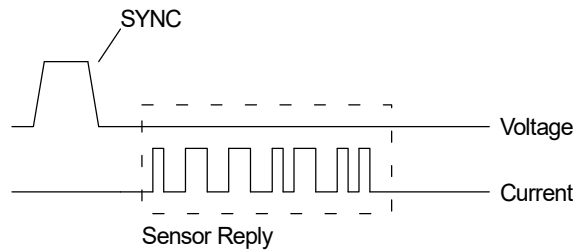
Figure 7-4 : PSI5 Diagram
