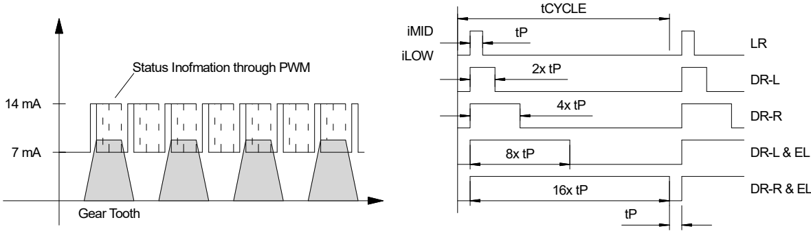
Figure 7-2 : PWM Diagram
