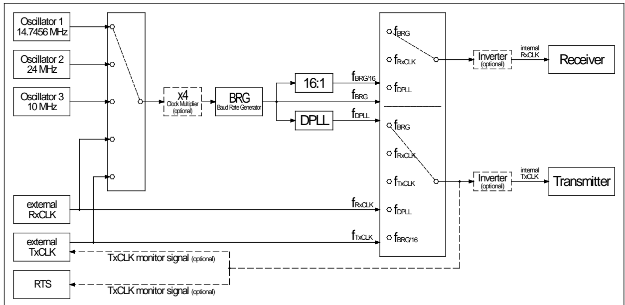
Figure 4-2 : Clock Sources
