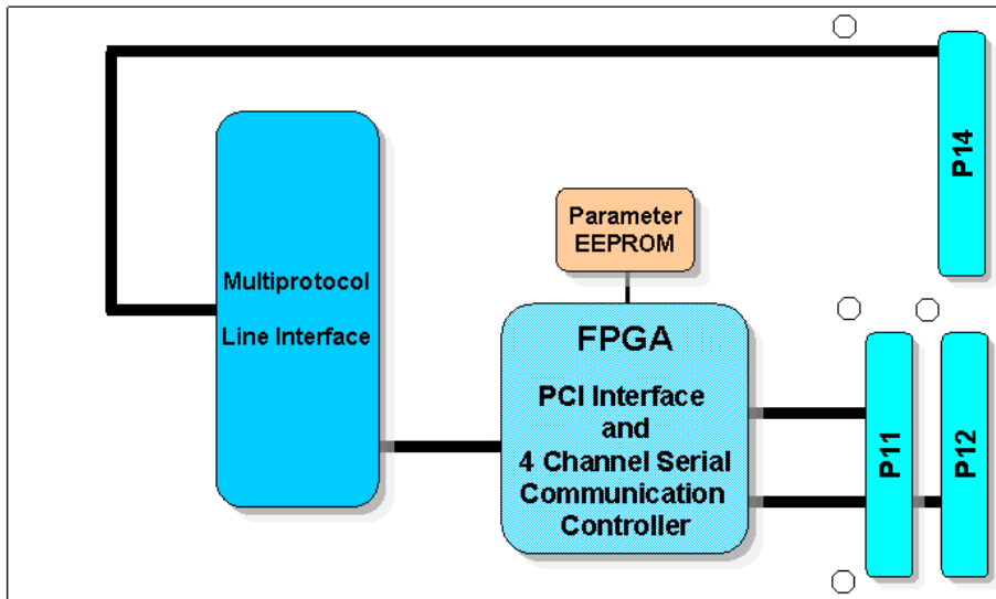
Figure 1-1 : Block Diagram
