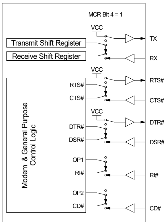
Figure 5-1 : Internal Loopback Connections
