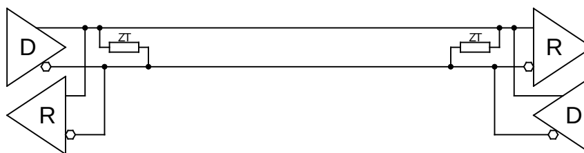
Figure 5-7: RS485 Half Duplex Point to Point Configuration
