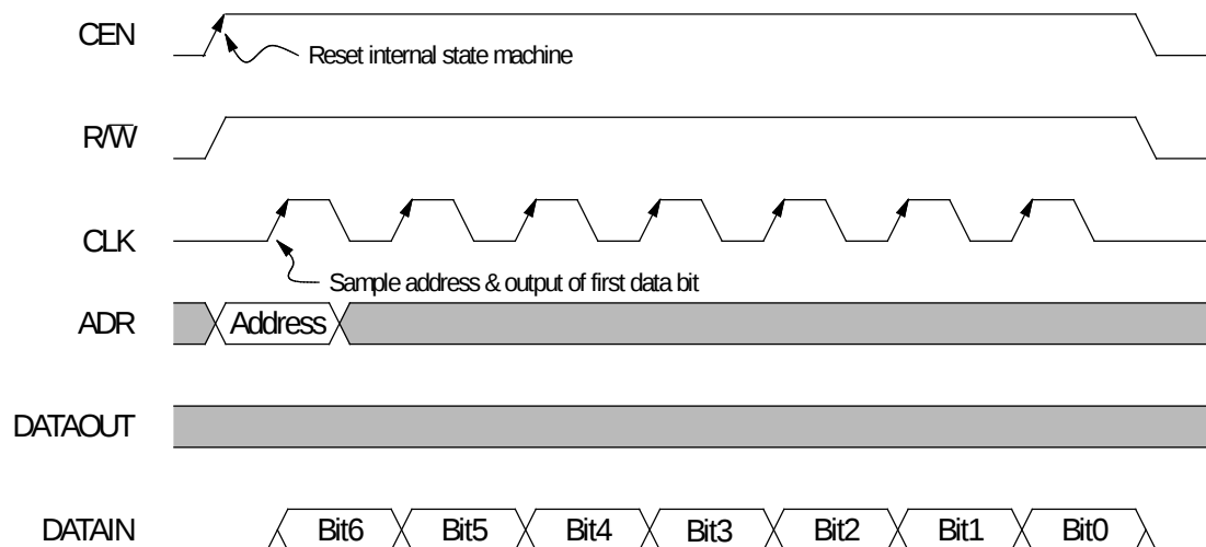
Figure 5-3 : CPLD-Bus Read
