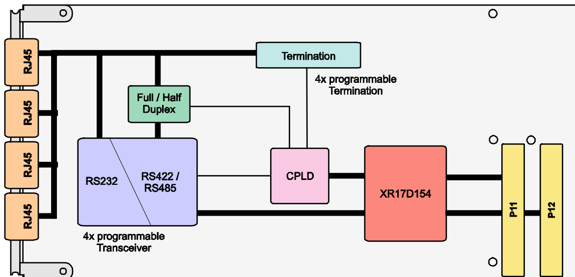
Figure 1-1 : Block Diagram
