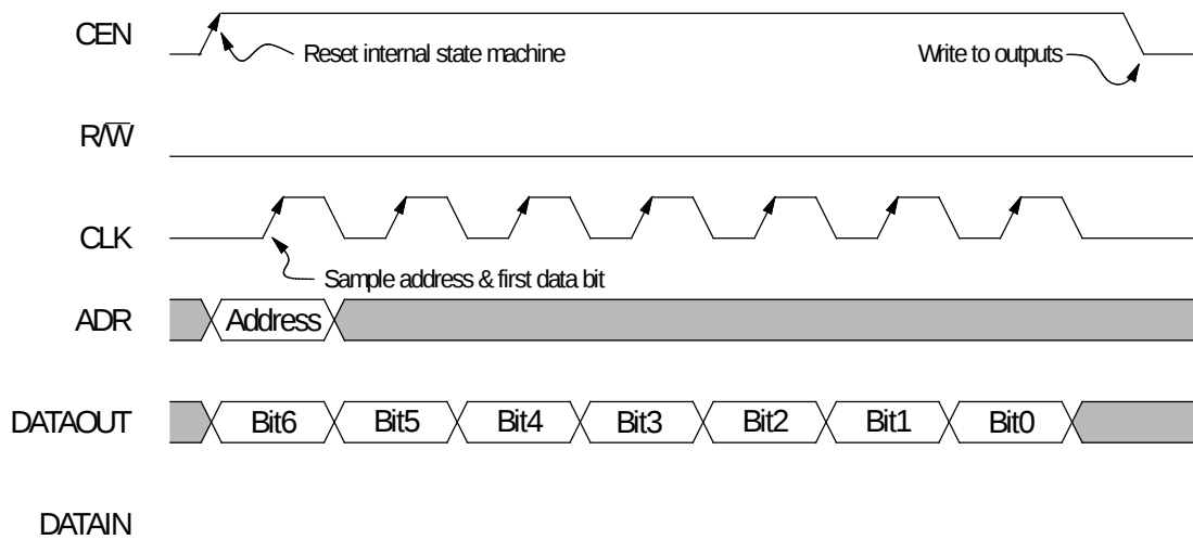
Figure 5-2 : CPLD-Bus Write
