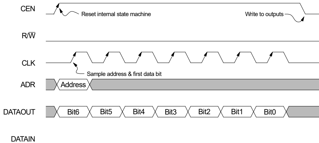
Figure 5-2 : CPLD-Bus Write
