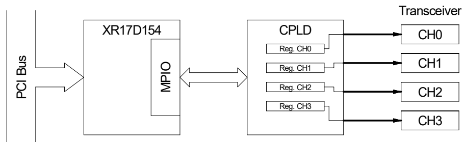
Figure 5-1 : CPLD-Bus Block Diagram
