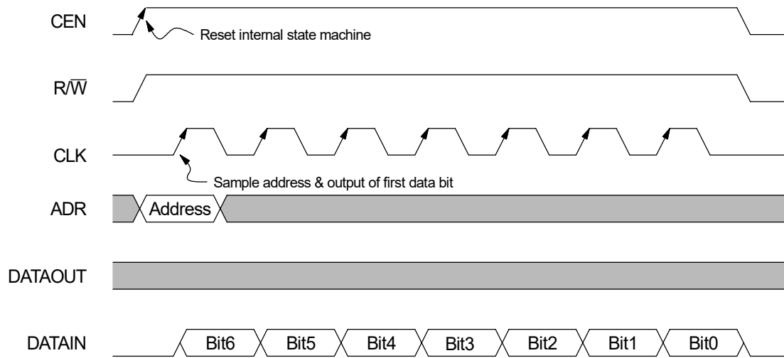
Figure 5-3 : CPLD-Bus Read
