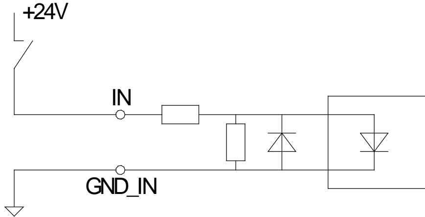
Figure 7-1 : Input Wiring
