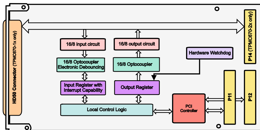
Figure 1-1 : Block Diagram
