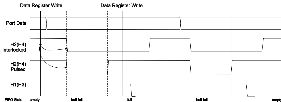
Figure 3-4 : Output Transfer Timing Diagram
