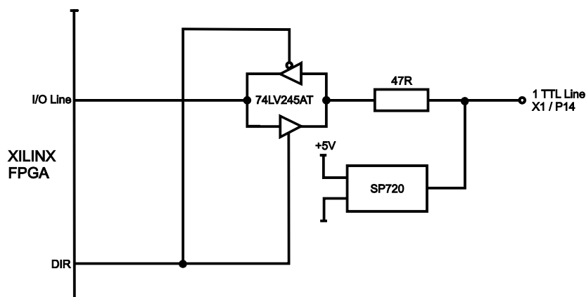
Figure 7-1 : I/O Circuitry
