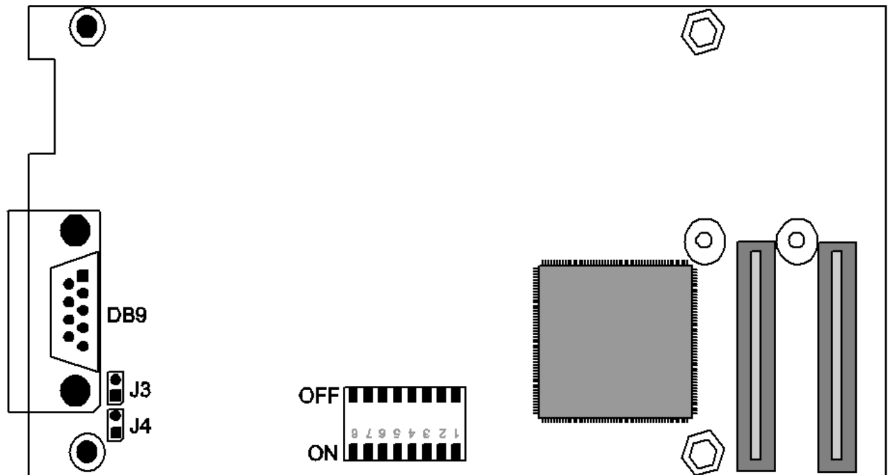
Figure 7-1 : Jumper Location
