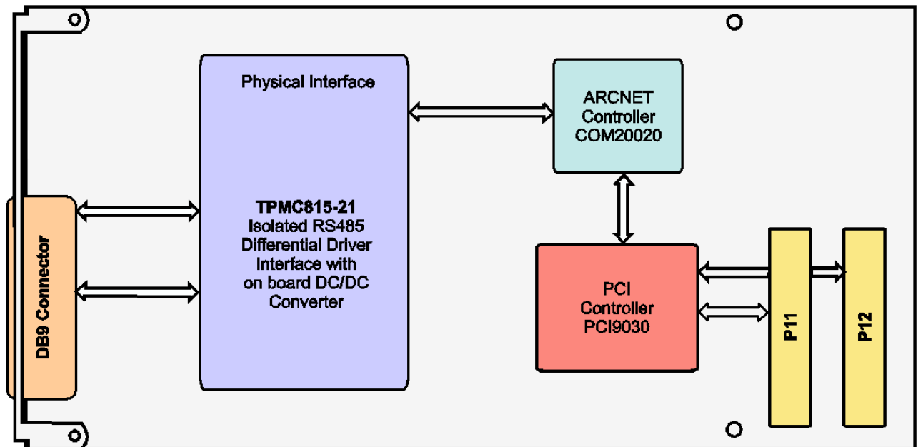
Figure 1-1 : Block Diagram
