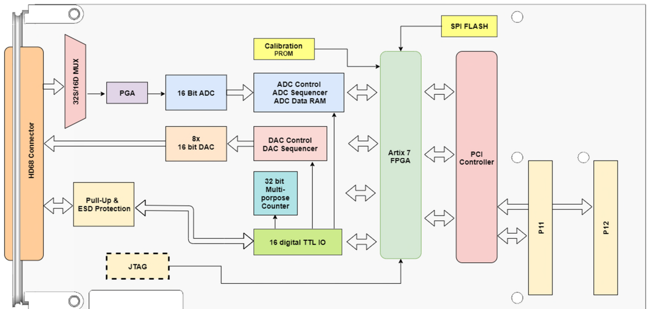
Figure 1-1 : Block Diagram
