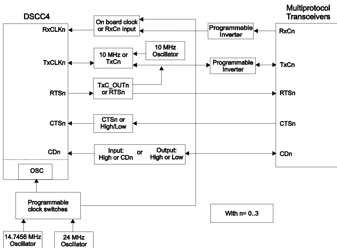
Figure 5-1 : Clock Sources
