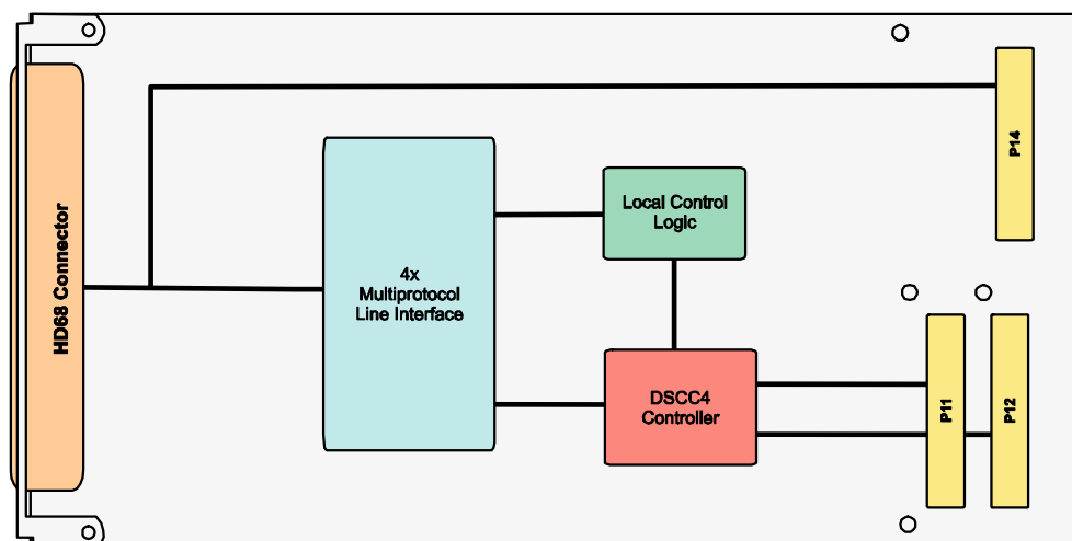
Figure 1-1 : Block Diagram
