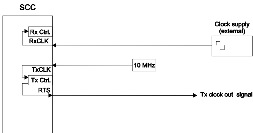
Figure 5-9 : Clock Mode 9
