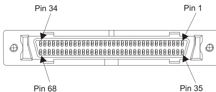
Figure 6-1 : Front Panel I/O Connector Numbering
