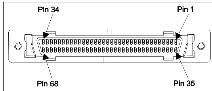
Figure 8-1 : Front Panel I/O Connector Numbering
