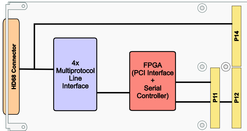
Figure 1-1 : Block Diagram
