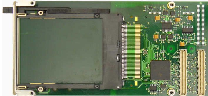
TPMC872-20 component side
