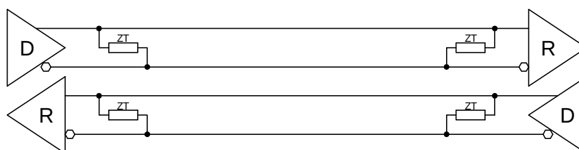
Figure 7-3 : RS485 Full Duplex Point to Point Configuration
