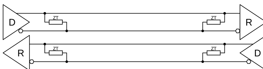
Figure 7-3 : RS485 Full Duplex Point to Point Configuration
