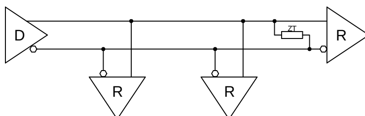
Figure 7-1 : RS422 Multidrop Configuration
