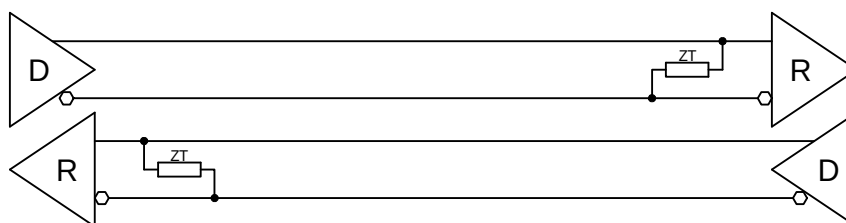
Figure 7-2 : RS422 Full Duplex Point to Point Configuration
