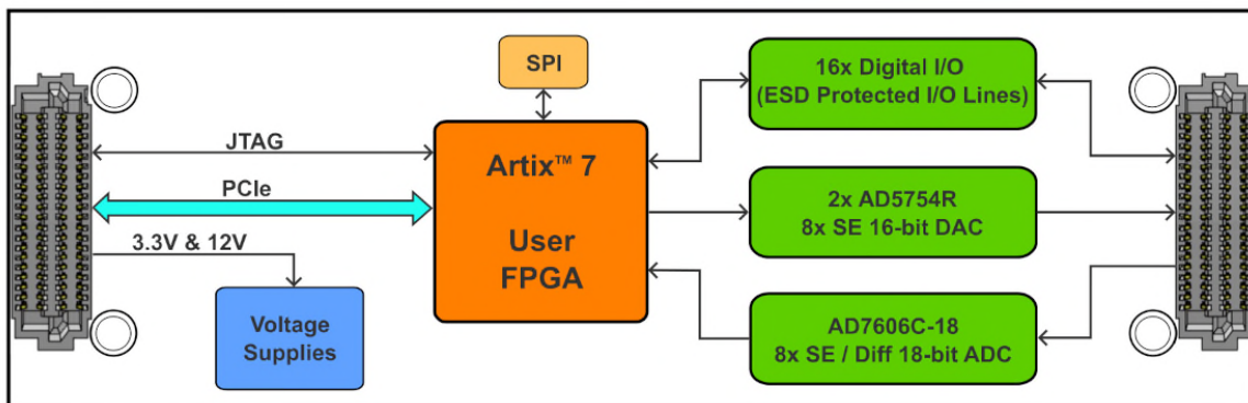
Block Diagram
