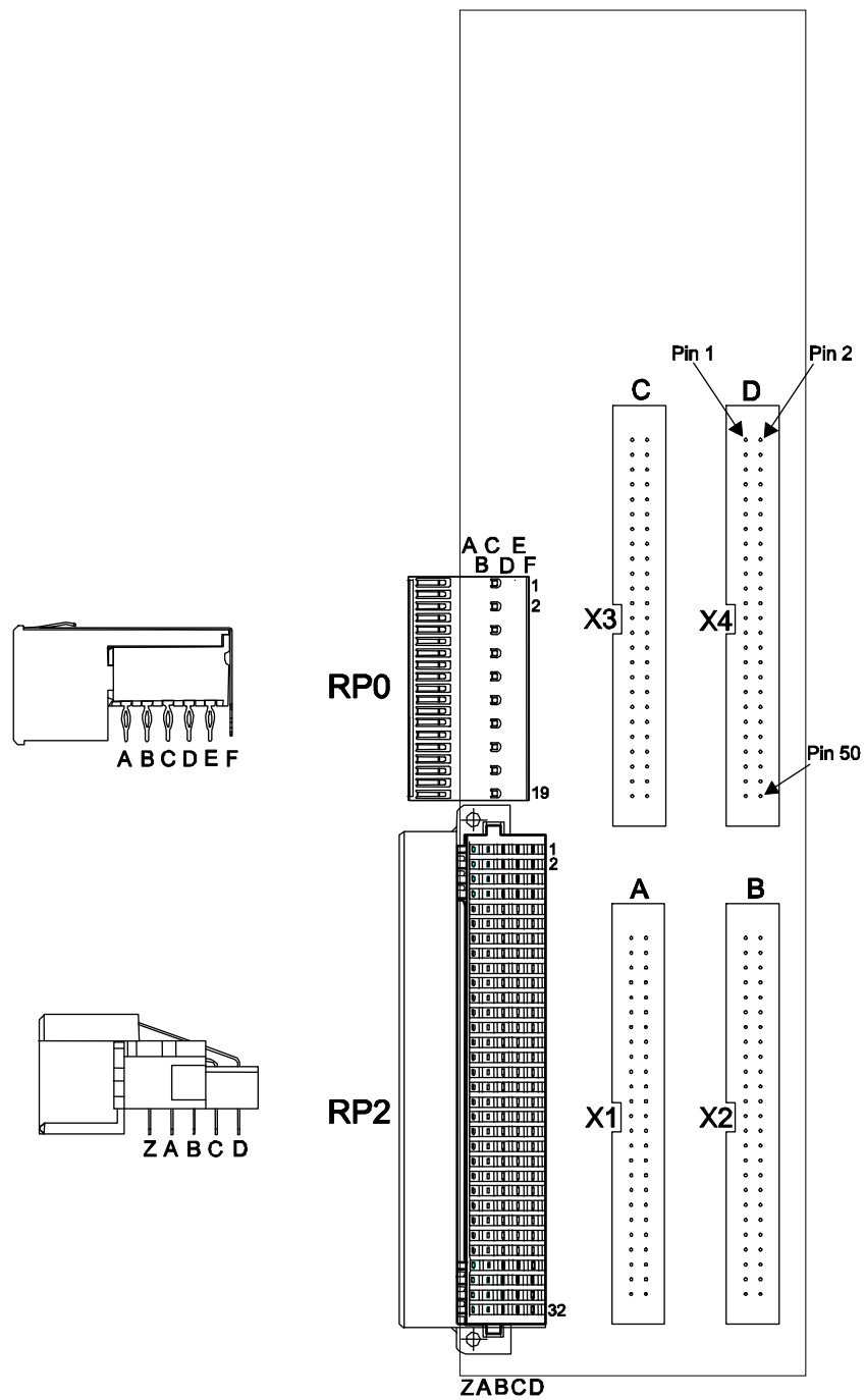
Figure 9-1 : Pin Assignment
