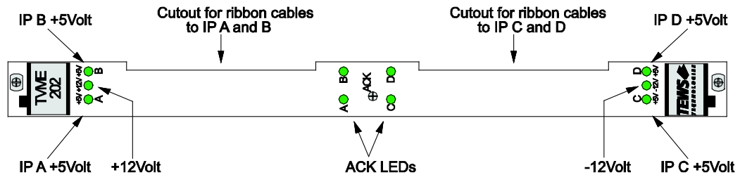
Figure 7-1 : Front Panel
