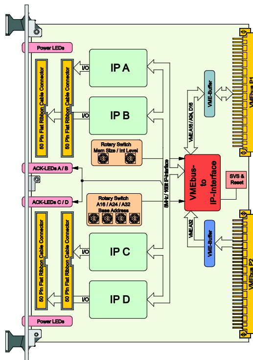
Figure 1-1 : Block Diagram
