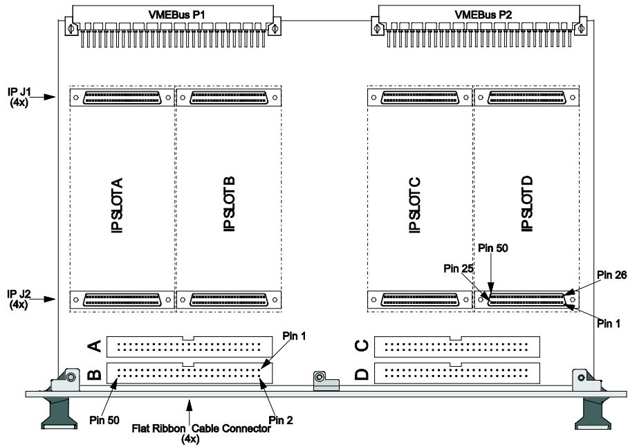
Figure 8-1 : Connector Overview
