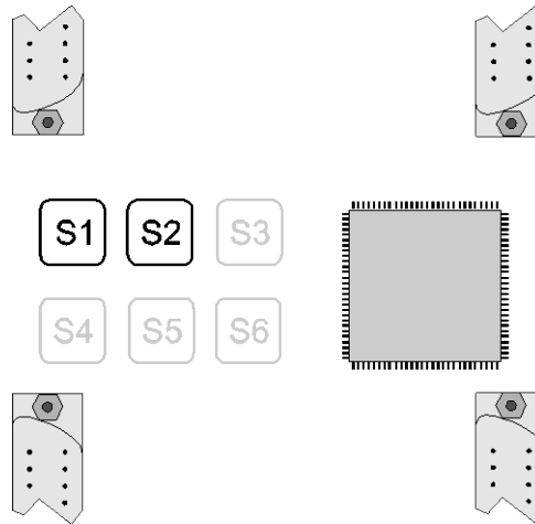
Figure 3-2 : VME A16 Base Address
