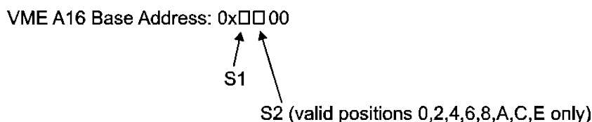
Figure 3-2 : VME A16 Base Address
