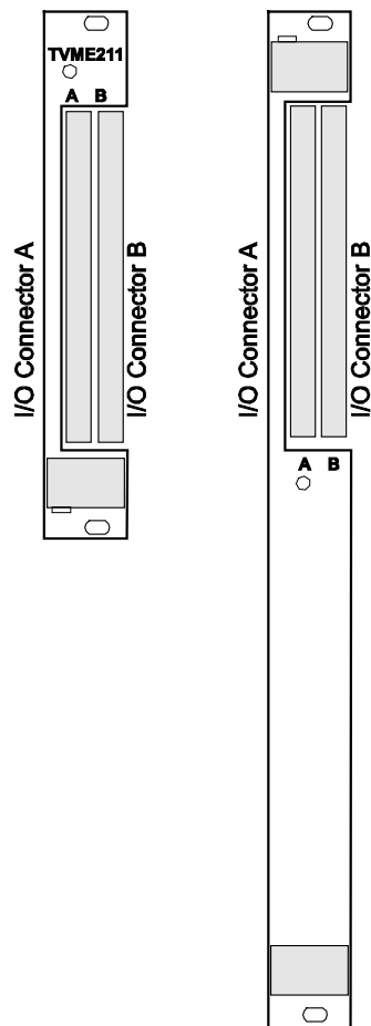
Figure 6-1 : Front Panel
