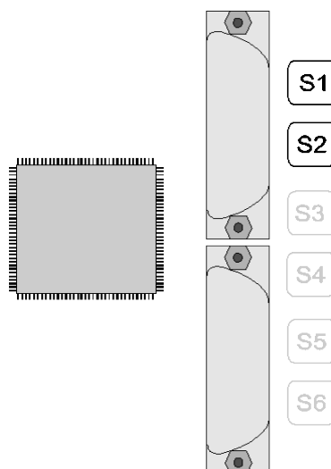
Figure 3-2 : VME A16 Base Address
