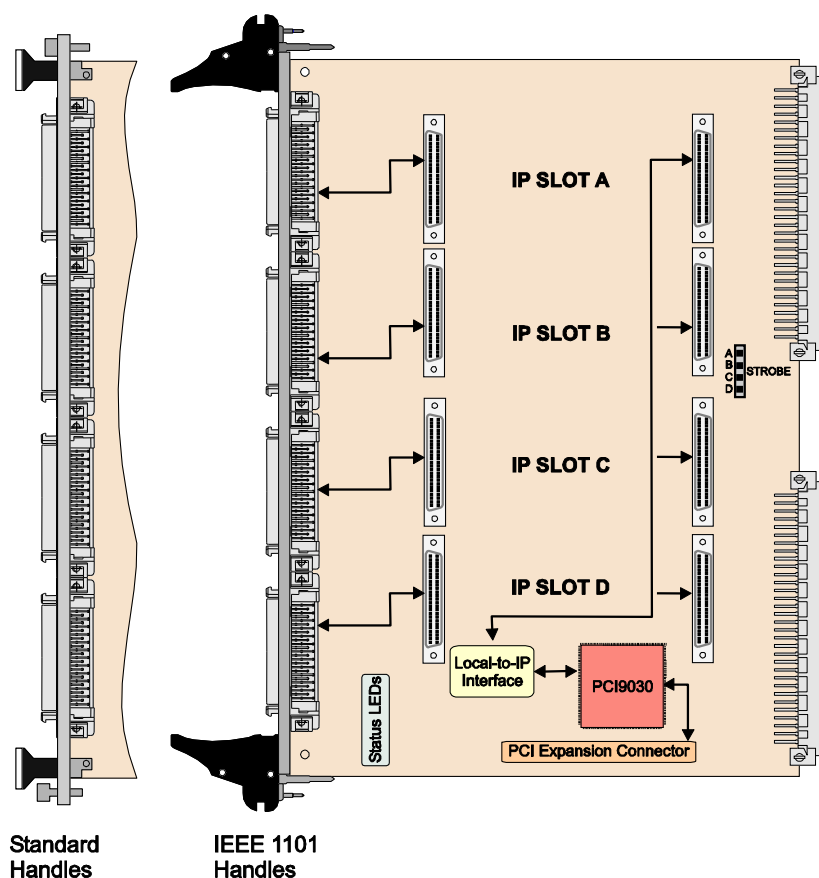
Figure 1-1 : Block Diagram
