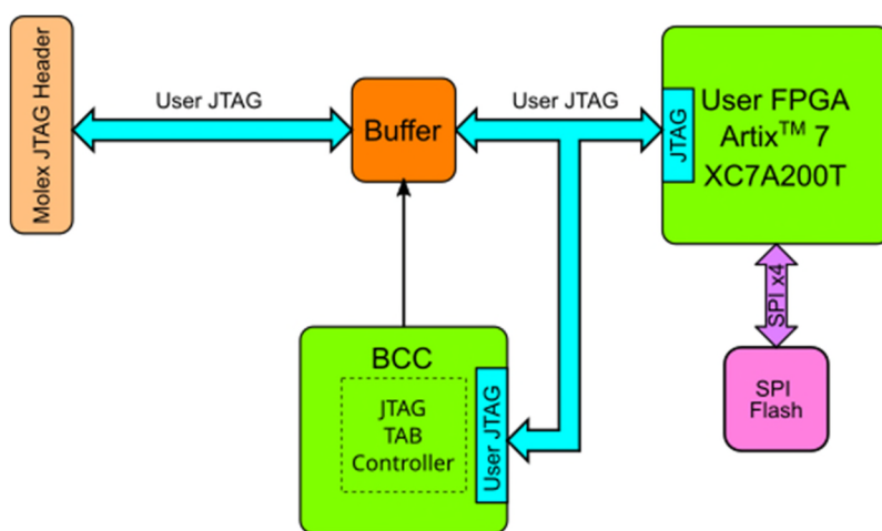
Figure 7-3 : User JTAG-Chain
