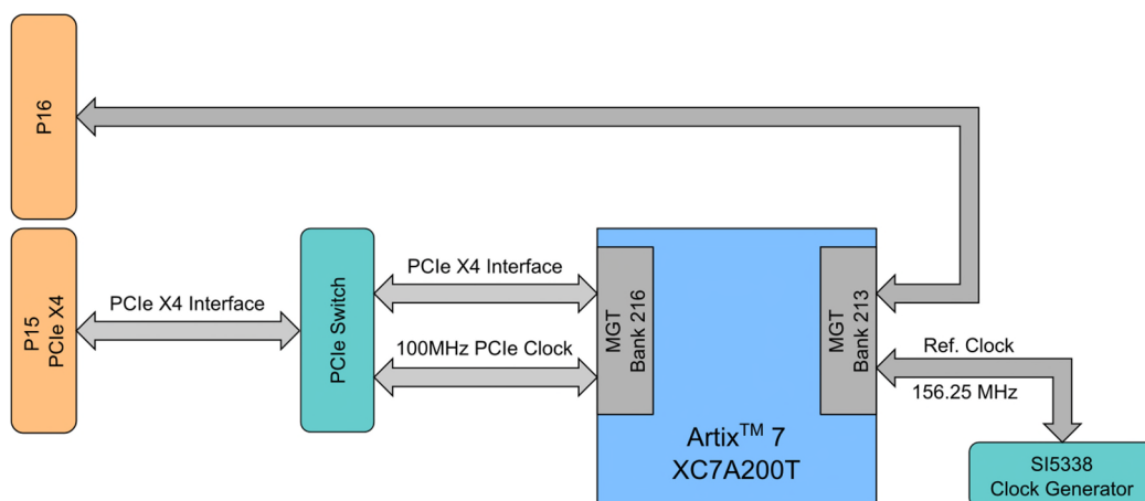
Figure 7-2 : User FPGA MGT Block Diagram
