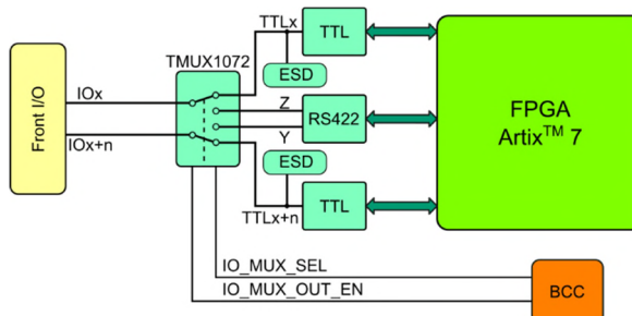
Figure 7-11 : 1 Channel Digital I/O Multiplexer Block Diagram
