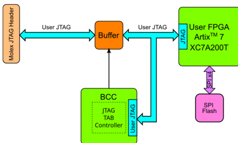
Figure 7-3 : User JTAG-Chain
