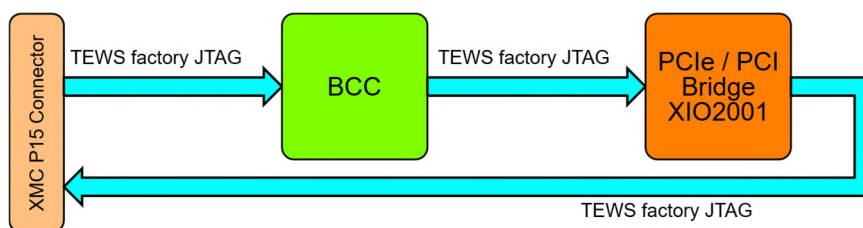
Figure 7-4 : TEWS Factory JTAG-Chain
