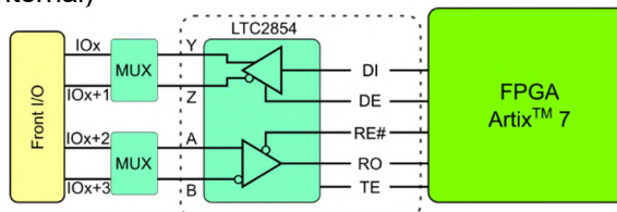
Figure 7-12 : One Channel RS422 I/O Interface
