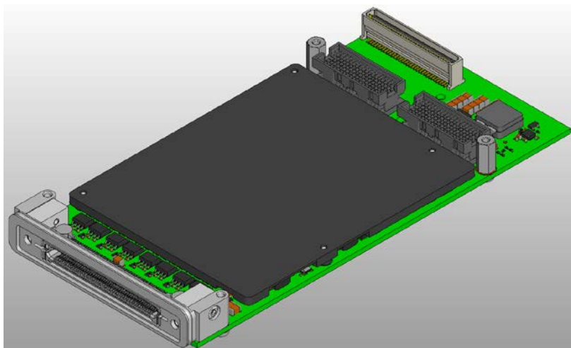
Figure 7-15: TXMC638 with Heatsink
