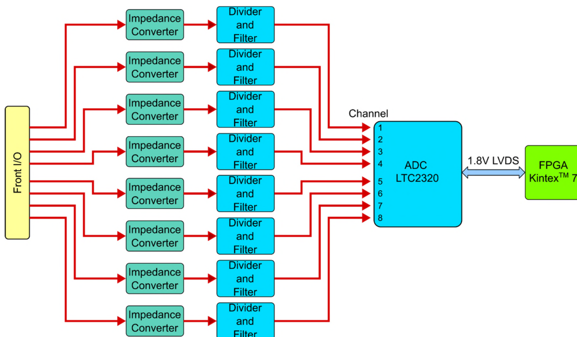
Figure 7-7 : Analog Input Block Diagram
