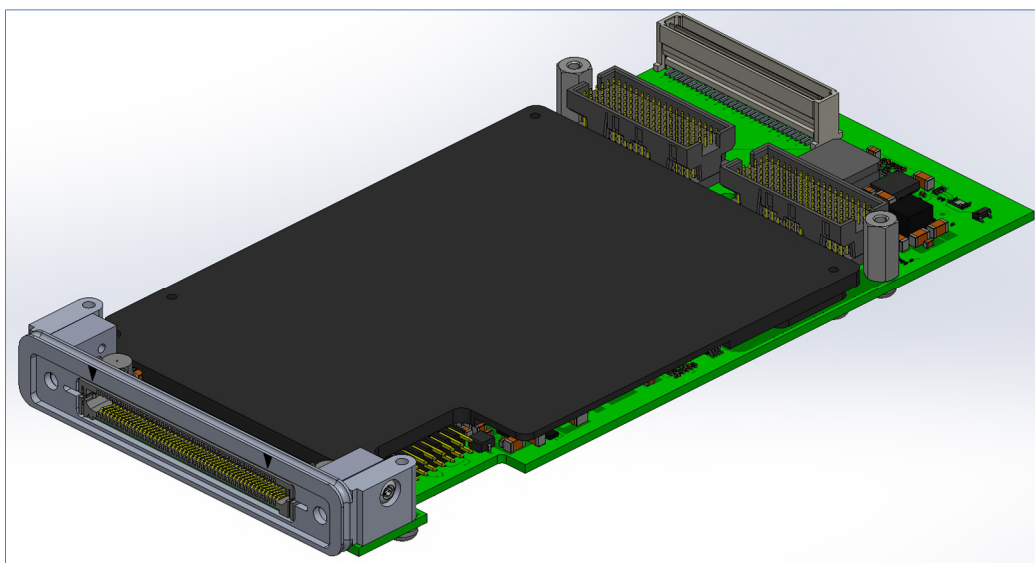
Figure 7-16: TXMC639 with Heatsink
