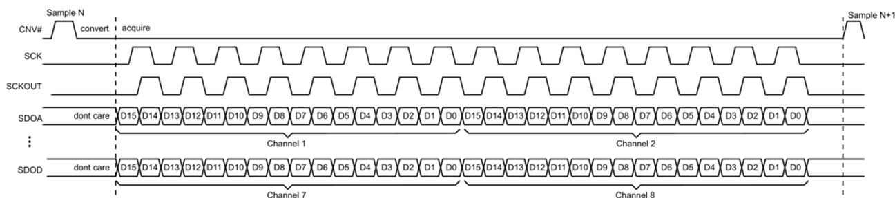
Figure 7-9 : Timing Diagram LTC2320-16 DDR-Mode (2 Channels per SDO Pair)
