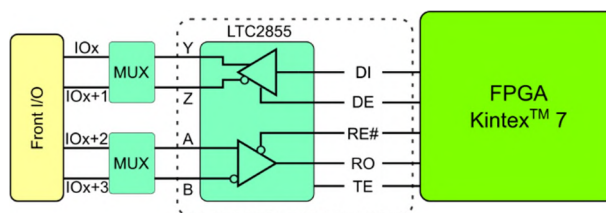
Figure 7-14 : One Channel RS422 I/O Interface
