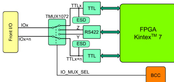
Figure 7-13 : 1 Channel Digital I/O Multiplexer Block Diagram
